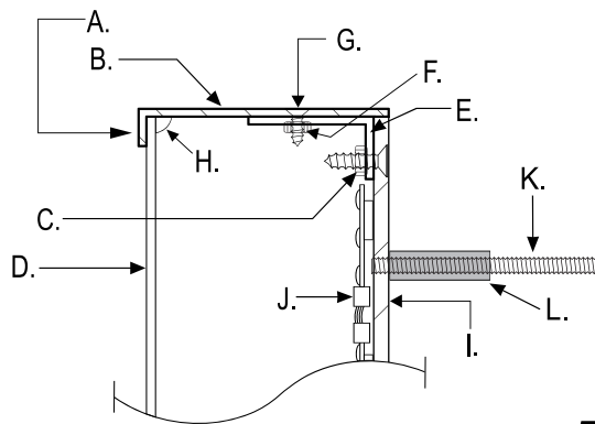
Side View Section Detail:
